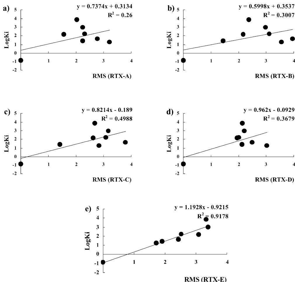
Figure 4. Correlation between rms and binding affinity.
