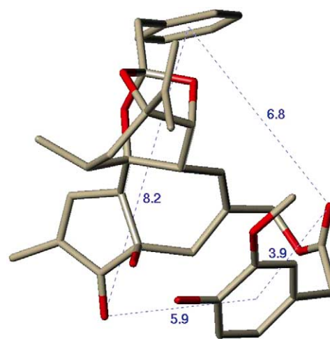
Figure 6. Proposed active conformation of RTX (RTX-E).
